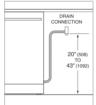
Drain connection
