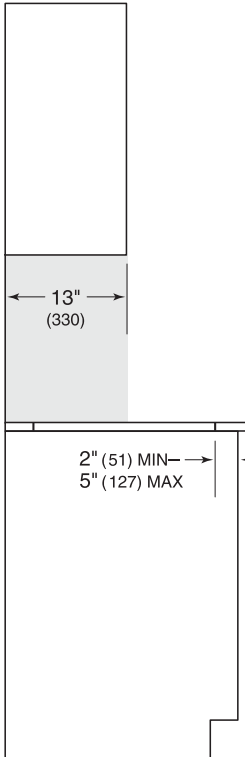
SIDE VIEW
