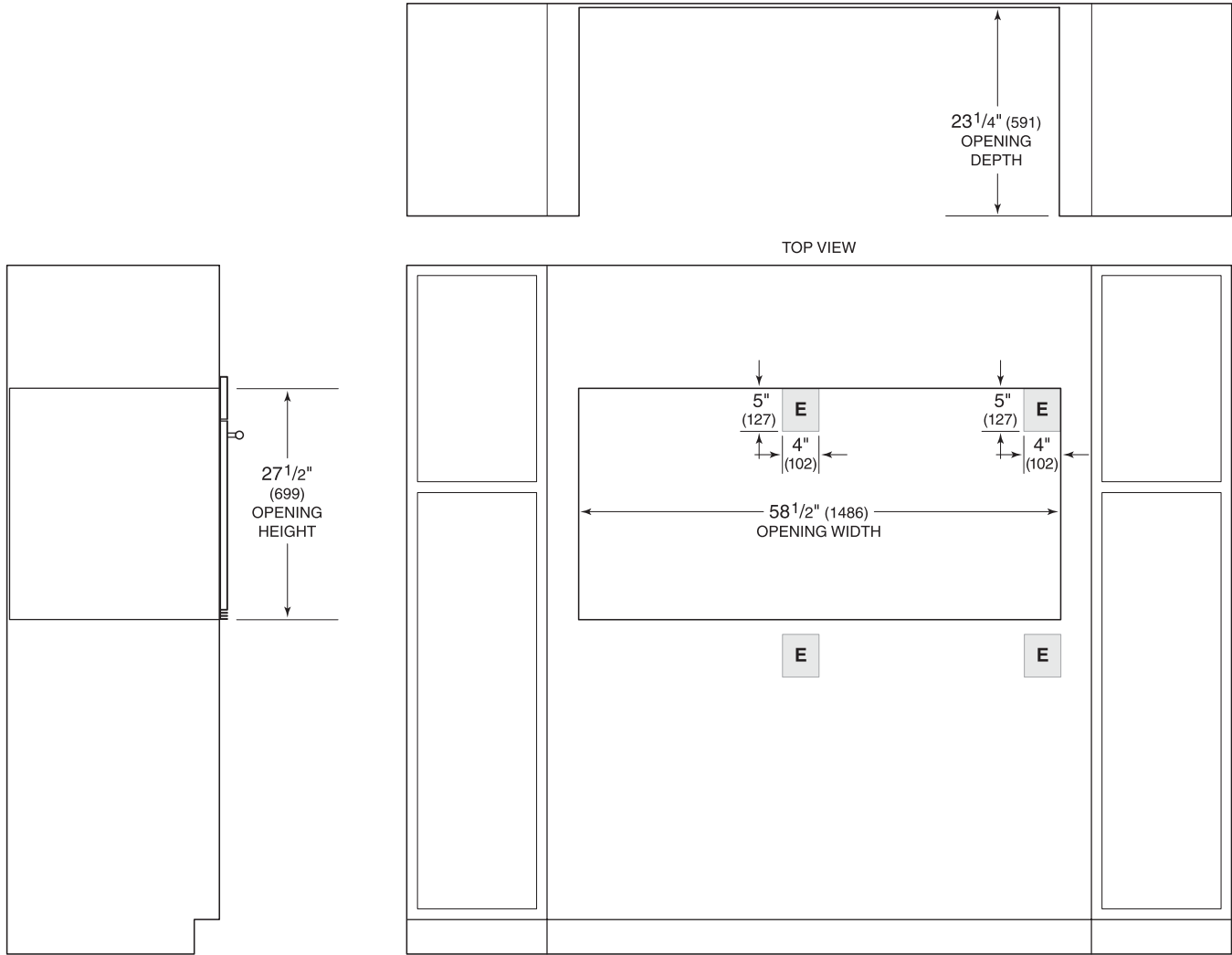
SIDE VIEW
